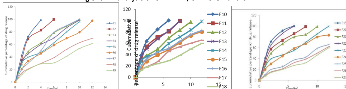
Fig 6: In-vitro dissolution profile of CEFIXIME, CEFACTOR and CEFDINIR
